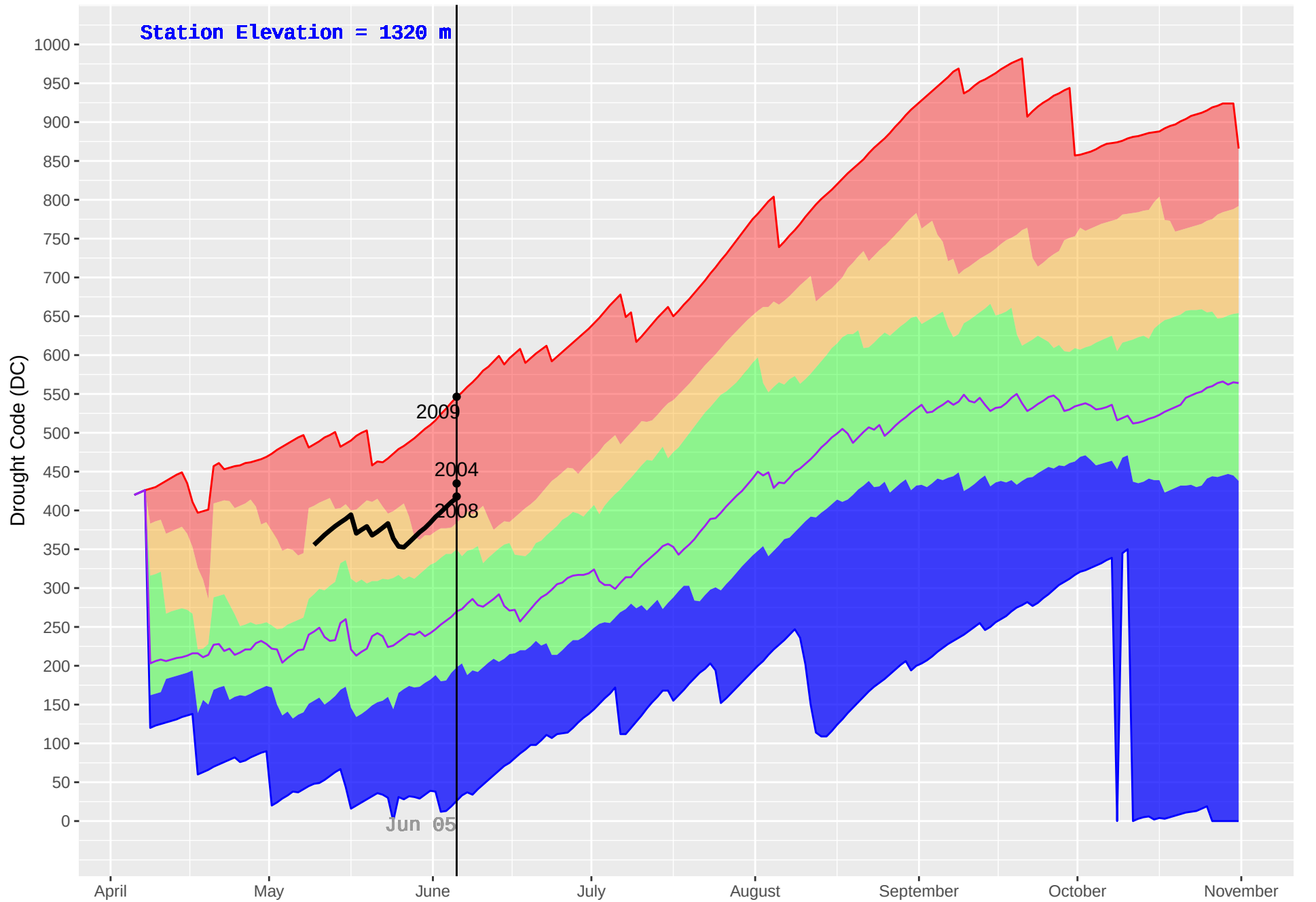
FRENCH BAR (306) : Historical (1979–2018) and Current (2019) Daily Drought Code (DC)
