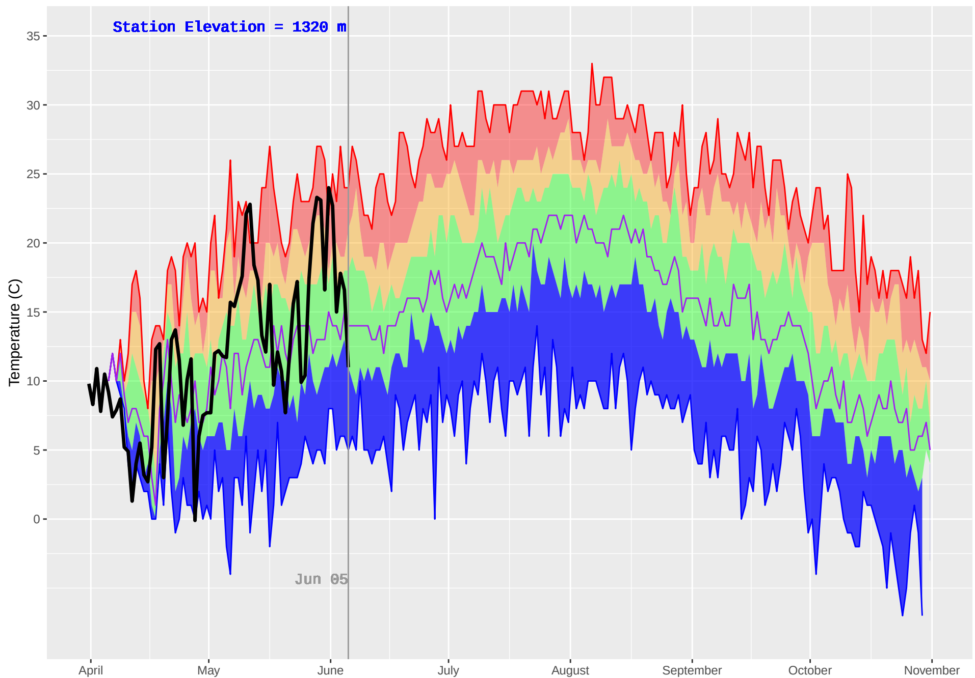
FRENCH BAR (306) : Historical (1979–2018) and Current (2019) Daily Temperature
