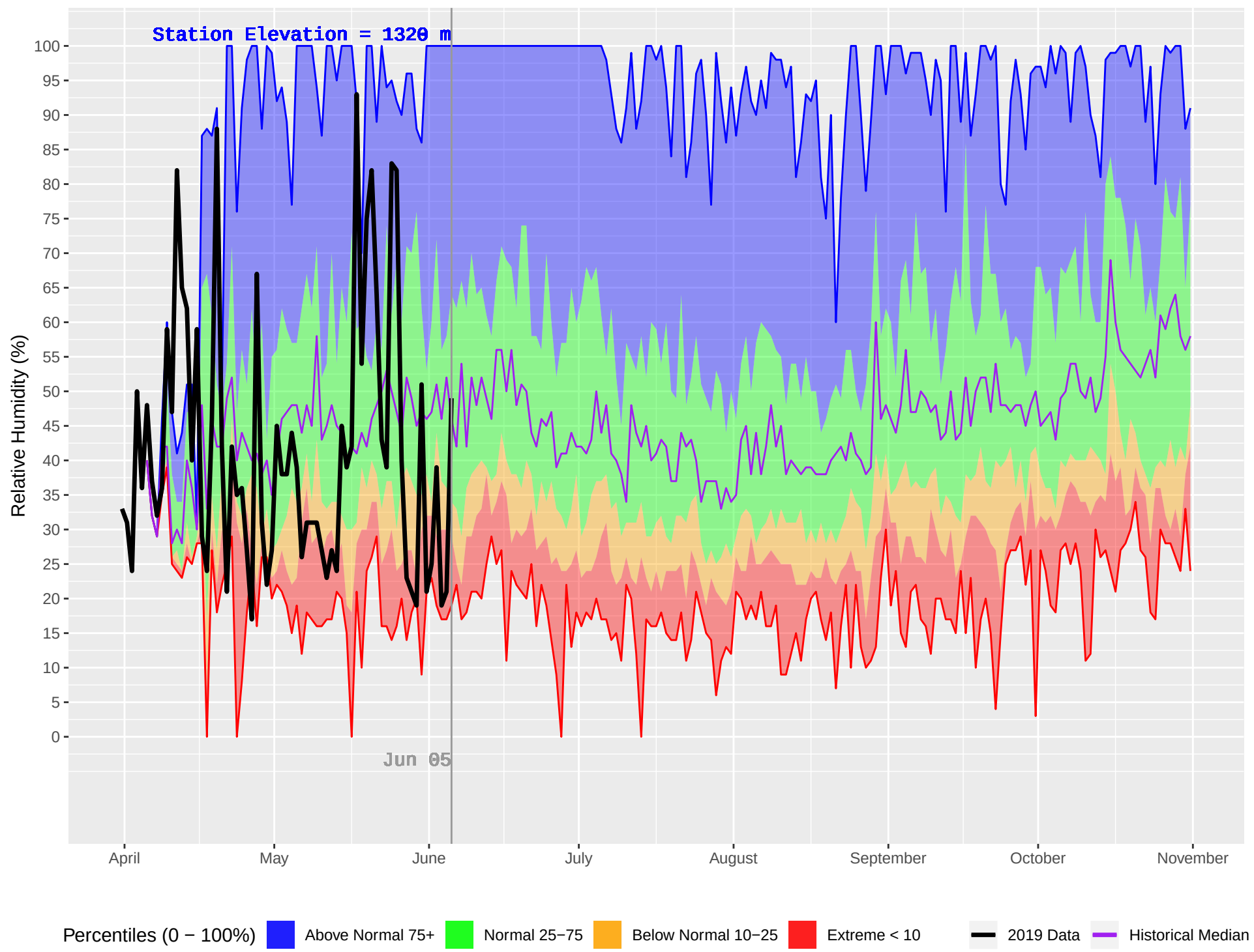
FRENCH BAR (306) : Historical (1979–2018) and Current (2019) Daily Relative Humidity
