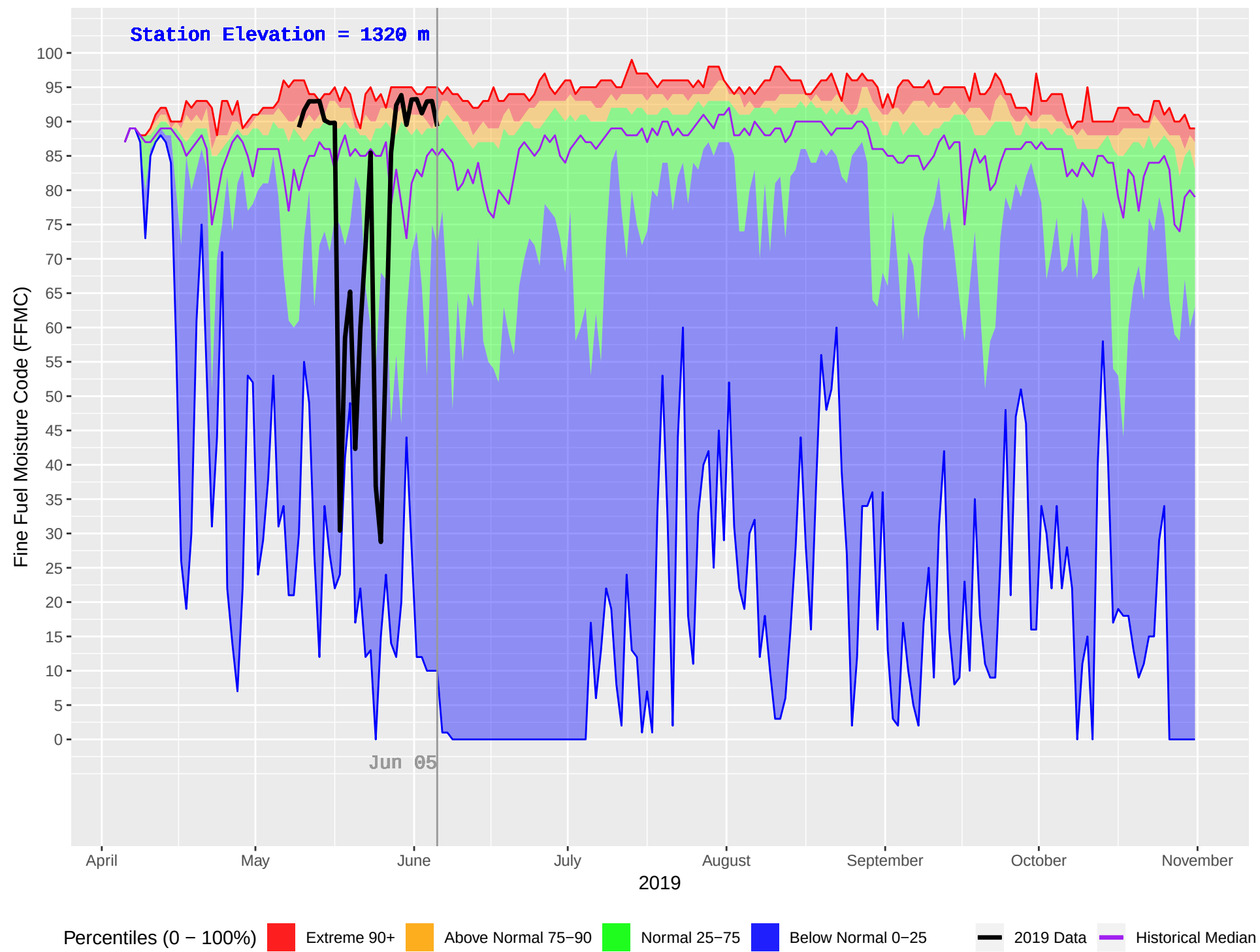
FRENCH BAR (306) : Historical (1979–2018) and Current (2019) Daily Fine Fuel Moisture Code (FFMC)
