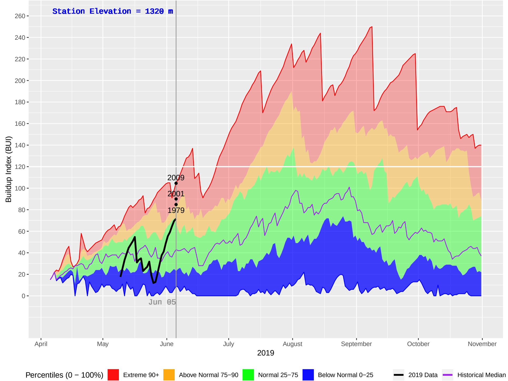
FRENCH BAR (306) : Historical (1979–2018), Current (2019) Daily Buildup Index (BUI)
