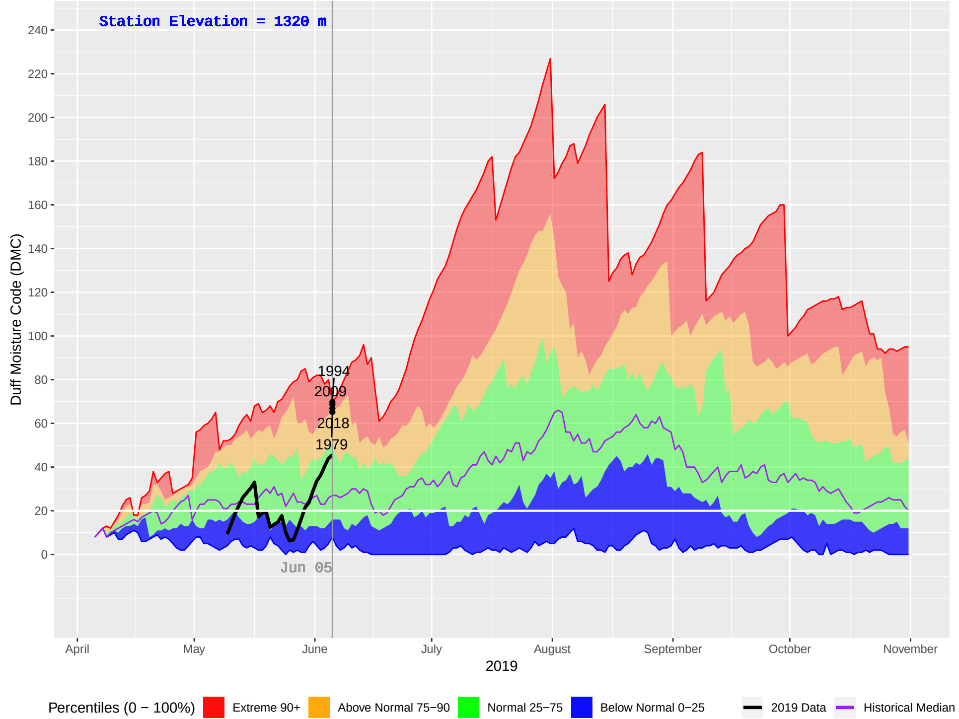
FRENCH BAR (306) : Historical (1979–2018), Current (2019) Daily Duff Moisture Code (DMC)
