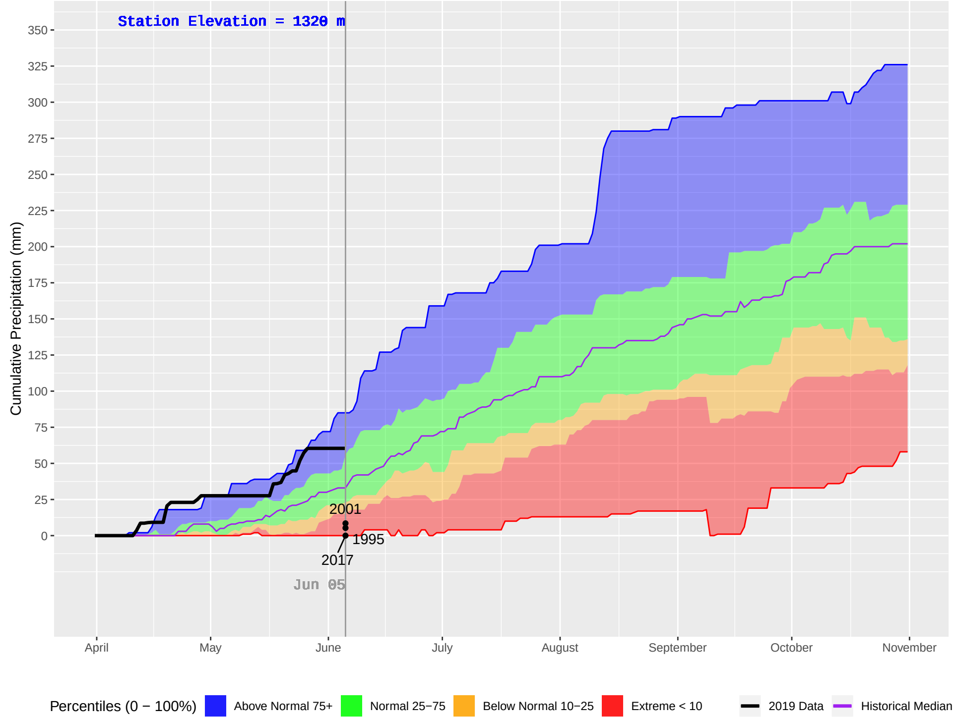
FRENCH BAR (306) : Historical (1979–2018), Current (2019) Daily Cumulative Precipitation
